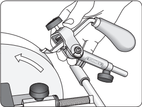
You can also grind a down bent gouge. The jig is set as shown on page 83.
