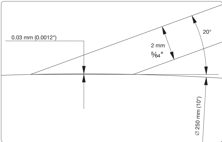
Ten times enlargement of a 2 mm thick tool ground with a 20^\circ edge angle. In spite of the enlarged scale the hollow is hardly noticeable. It is only 0.03 mm or 0.0012".
