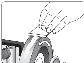
Start the machine and distribute the compound by pressing a tool gently against the wheel. Let the compound penetrate the leather.
