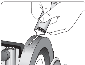
Apply a thin string of the compound before starting the machine. Rotate the wheel by hand.
