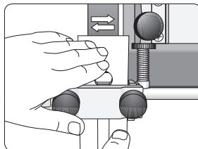
Honing a plane iron in the SVH-60 jig.
