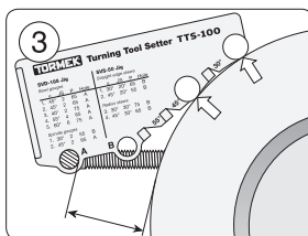
Set the Universal Support. Use hole A or hole B.
