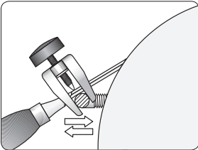
Setting the existing edge angle. Adjust the Universal Support so the entire bevel touches the grindstone. Use the Marker Method.
