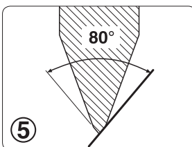
5 Another honing sharpens the edge to a still larger angle.
