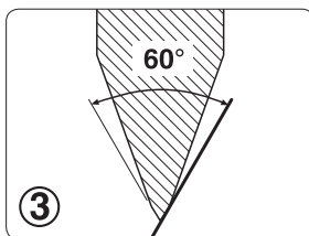
3 After honing on a bench stone the edge is sharp again, but with an increased edge angle.
